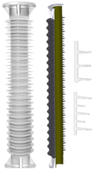
Composite hollow insulator
